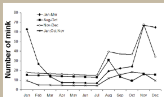
ABOVE: The graph shows the predicted number of mink in the control area throughout the year, depending on the period of the year that trapping is carried out. All strategies result in fairly low numbers of mink in the spring and early summer, but trapping only in January-March, or only in November - December (for instance), results in high numbers of mink in the autumn. Kits (young mink < 3 months old) are not included in the model calculations, juveniles (> 3 months old) are included 36 .
